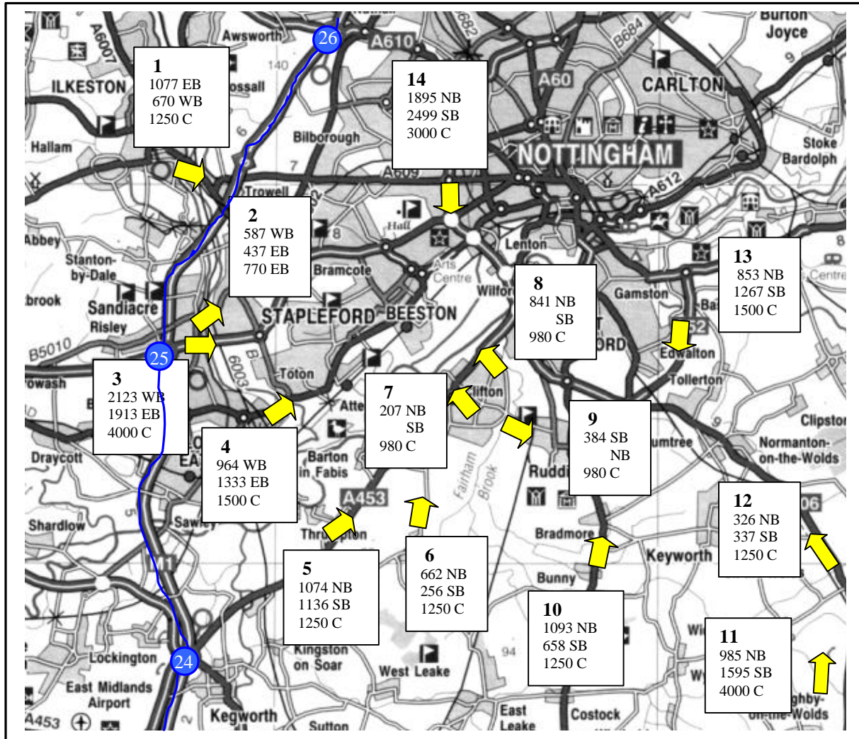
Figure 4.14 Two – Way Traffic Flow and Road Design Capacity During A.M. Peak for Base Year 2000
