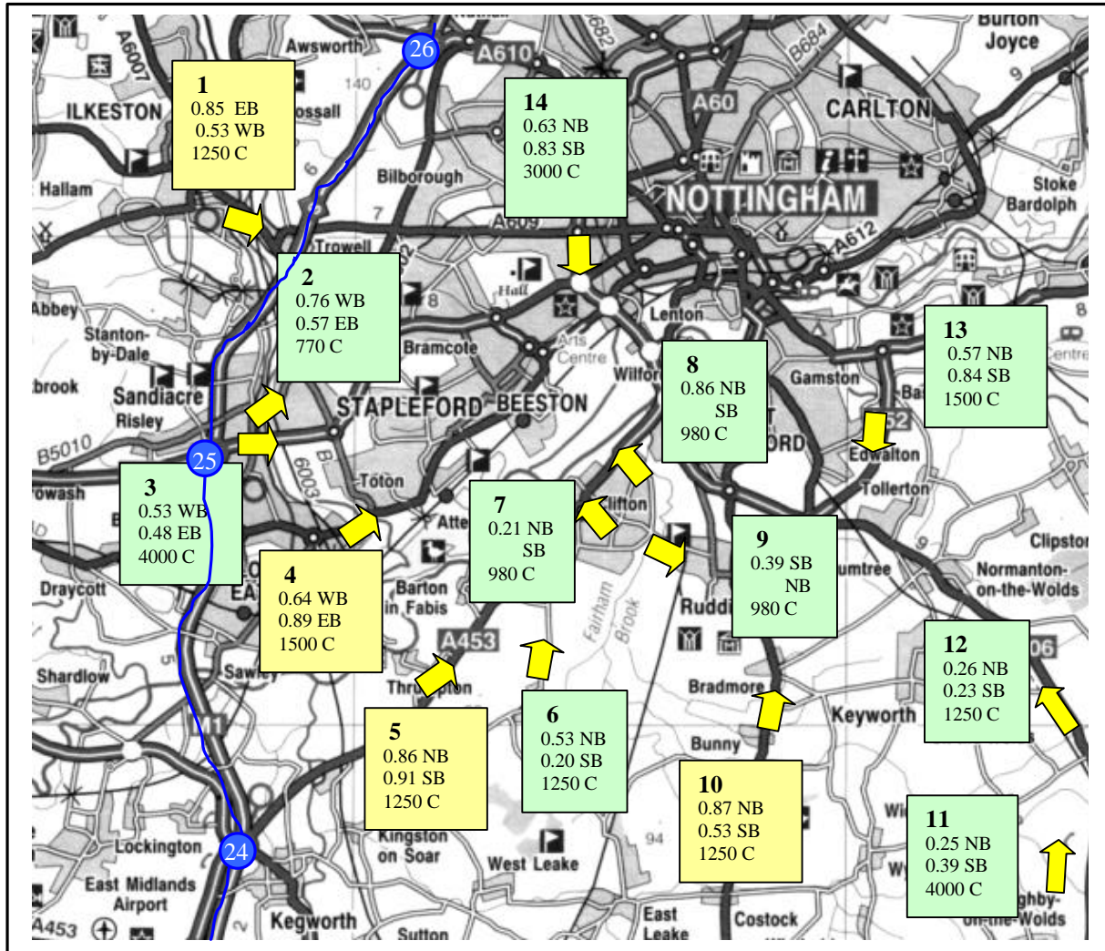
Figure 4.15 Ratio between Observed Flow and Road Design Capacity During A.M. Peak for Base Year 2000
