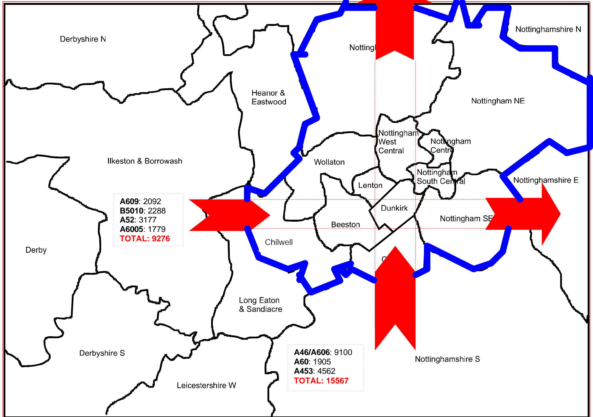
Fig 4.5 Through Traffic Movements (TTM)
