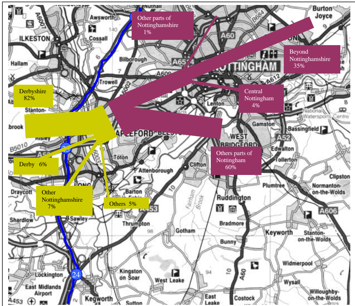
Figure 4.8 Select Link Analysis: B5010 Corridor
